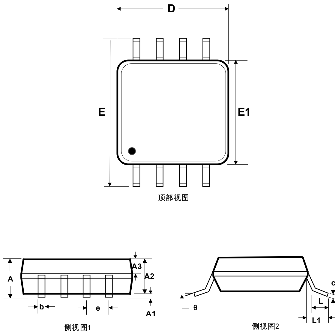
图11.2 IBSA1277-2 MSOP8封装尺寸
